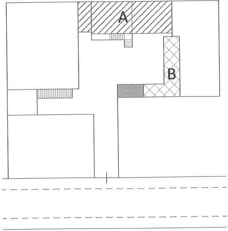
Planimetria (1:300)
